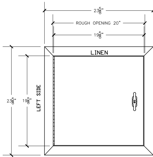
FRONT VIEW 20"X20" SIDE HINGED A/D U.L. APPROVED
