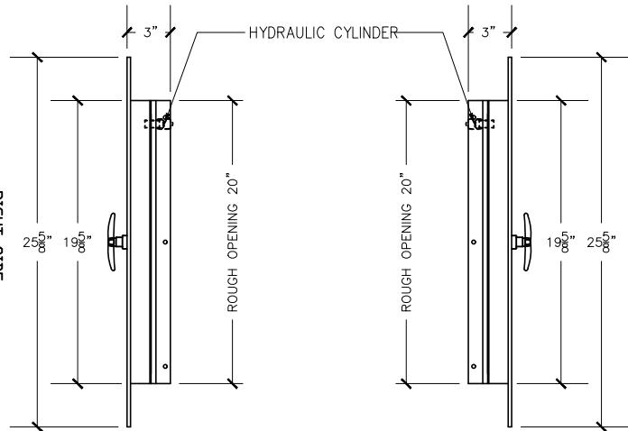
RIGHT VIEW
